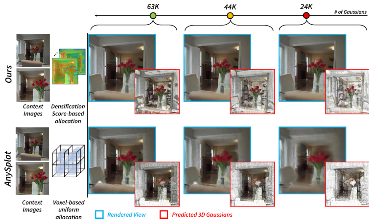
(a) Densification-score-guided allocation of F 4 Splat
