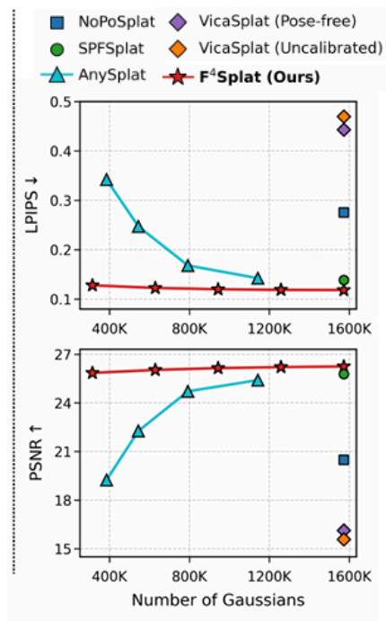
(b) Rendering quality vs. Number of Gaussians
